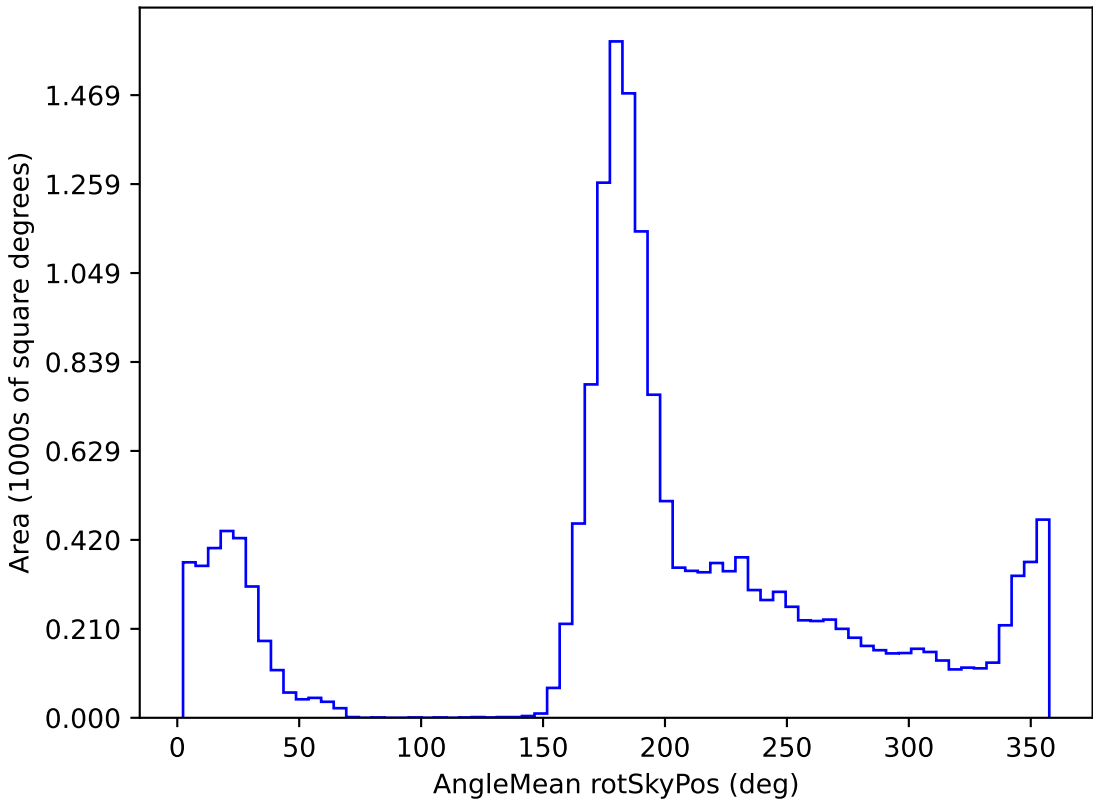
too_ignore_5_1v3.4_10yrs WFD g band: AngleMean rotSkyPos
