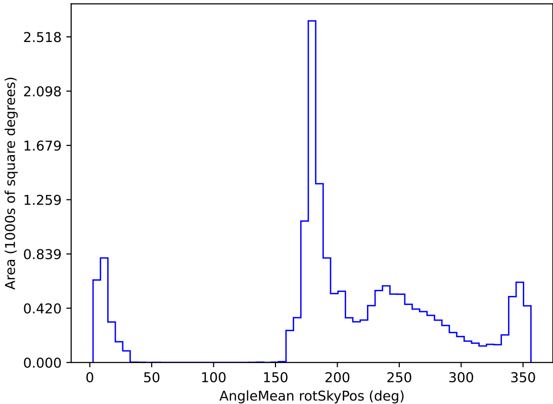
too_ignore_5_1v3.4_10yrs WFD all bands: AngleMean rotSkyPos
