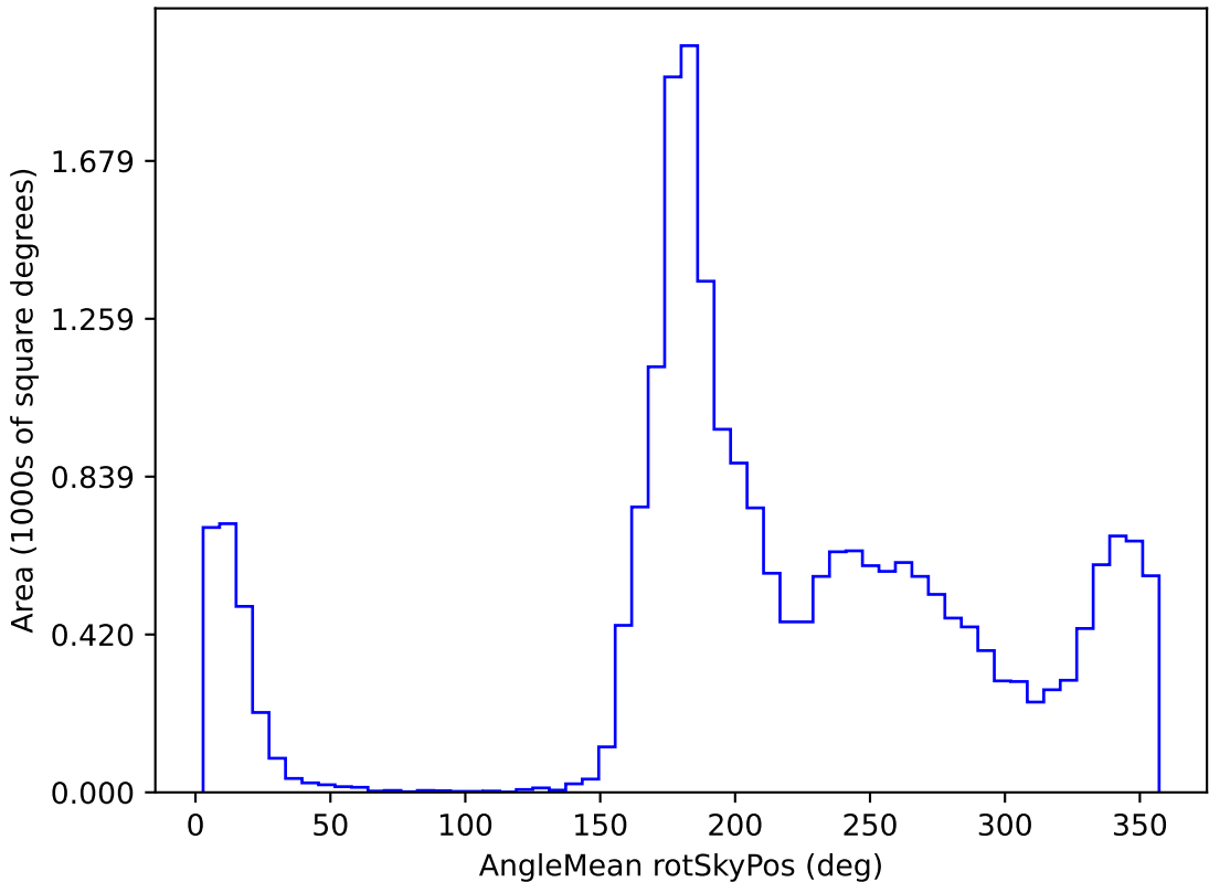
too_ignore_5_1v3.4_10yrs All sky y band: AngleMean rotSkyPos
