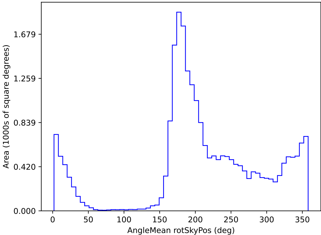
too_ignore_5_1v3.4_10yrs All sky u band: AngleMean rotSkyPos
