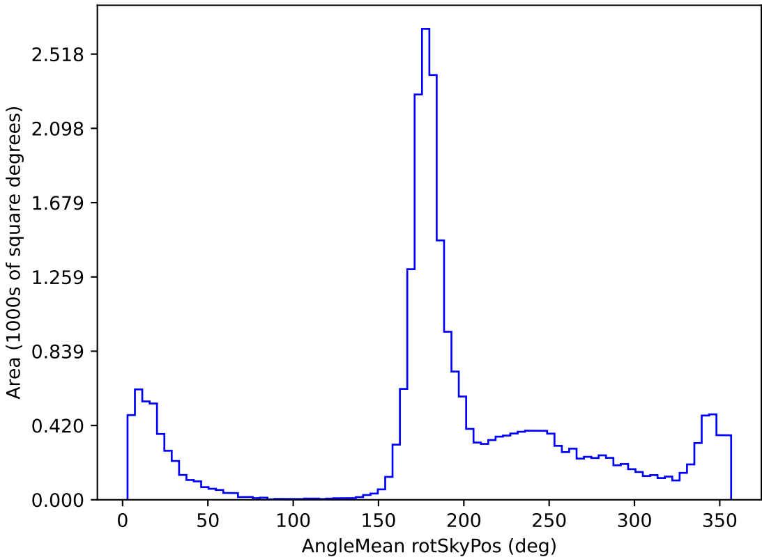
too_ignore_5_1v3.4_10yrs All sky r band: AngleMean rotSkyPos
