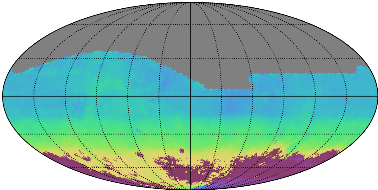
too_ignore_5_1v3.4_10yrs All sky i band: AngleMean rotSkyPos
