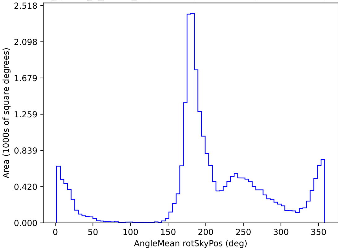
too_ignore_5_1v3.4_10yrs All sky i band: AngleMean rotSkyPos
