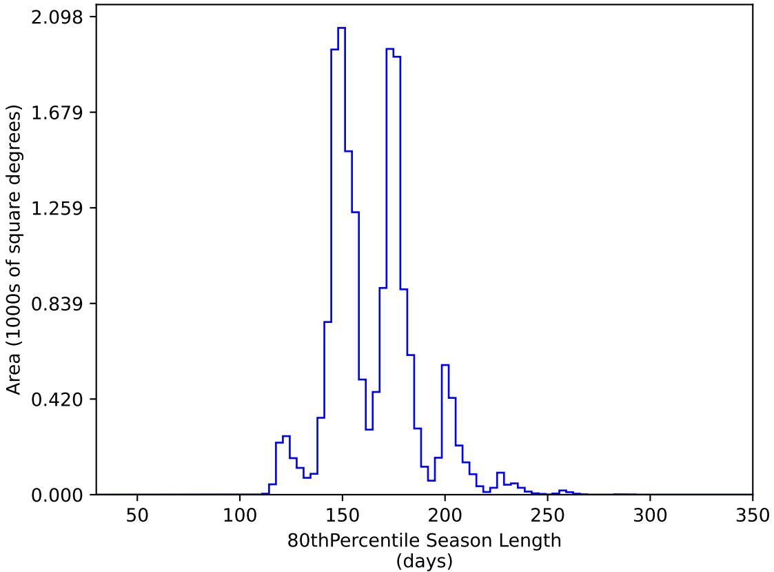
too_ignore_5_1v3.4_10yrs WFD y band: 80thPercentile Season Length
