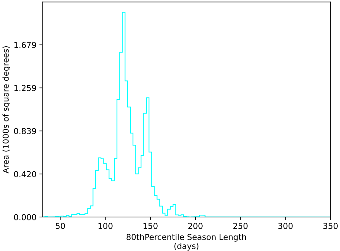
too_ignore_5_1v3.4_10yrs WFD u band: 80thPercentile Season Length
