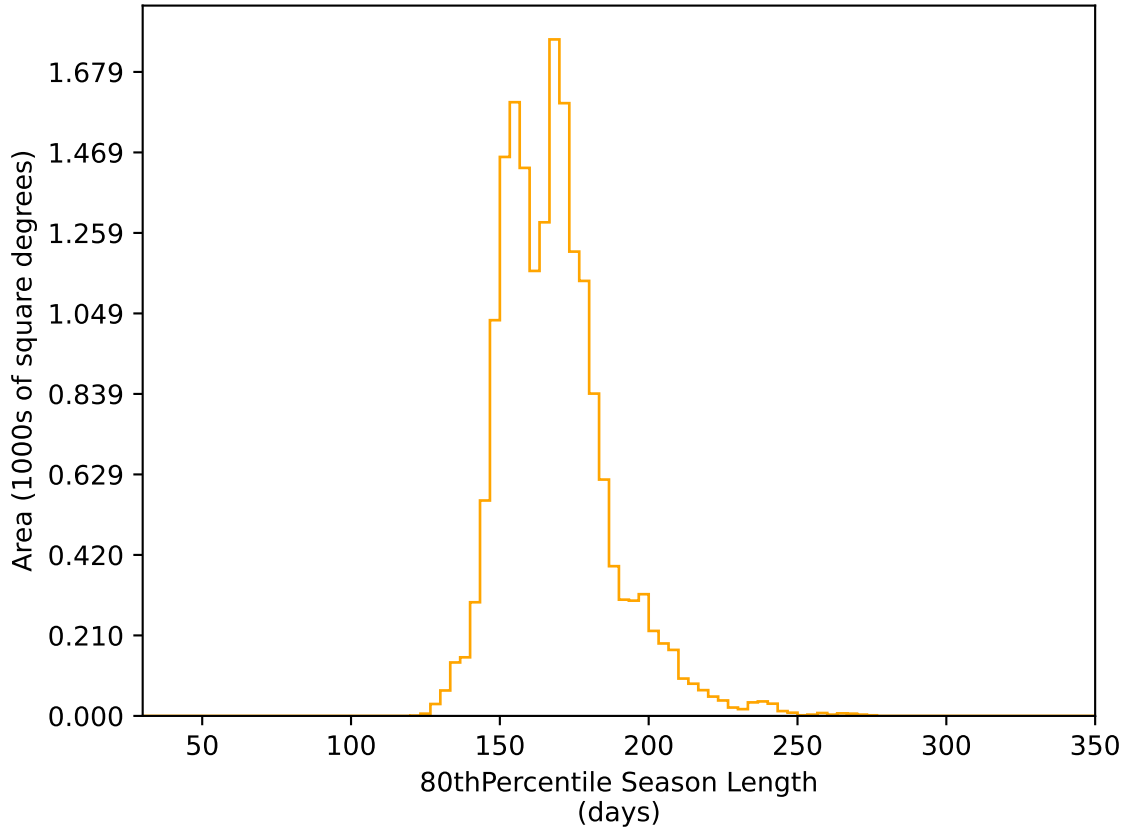
too_ignore_5_1v3.4_10yrs WFD r band: 80thPercentile Season Length
