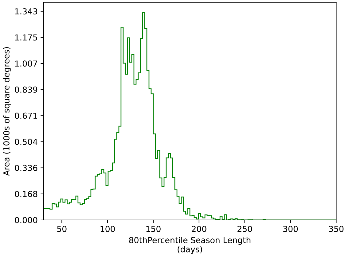
too_ignore_5_1v3.4_10yrs All sky g band: 80thPercentile Season Length
