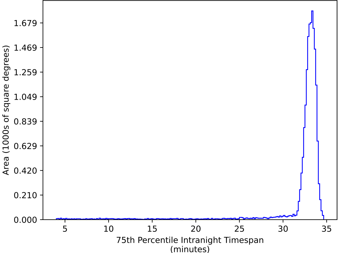
too_ignore_5_1v3.4_10yrs WFD ug bands: 75th Percentile Intranight Timespan
