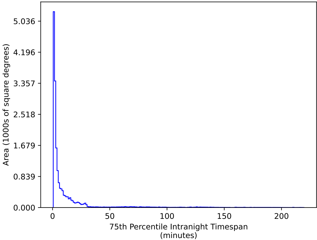
too_ignore_5_1v3.4_10yrs WFD u band: 75th Percentile Intranight Timespan
