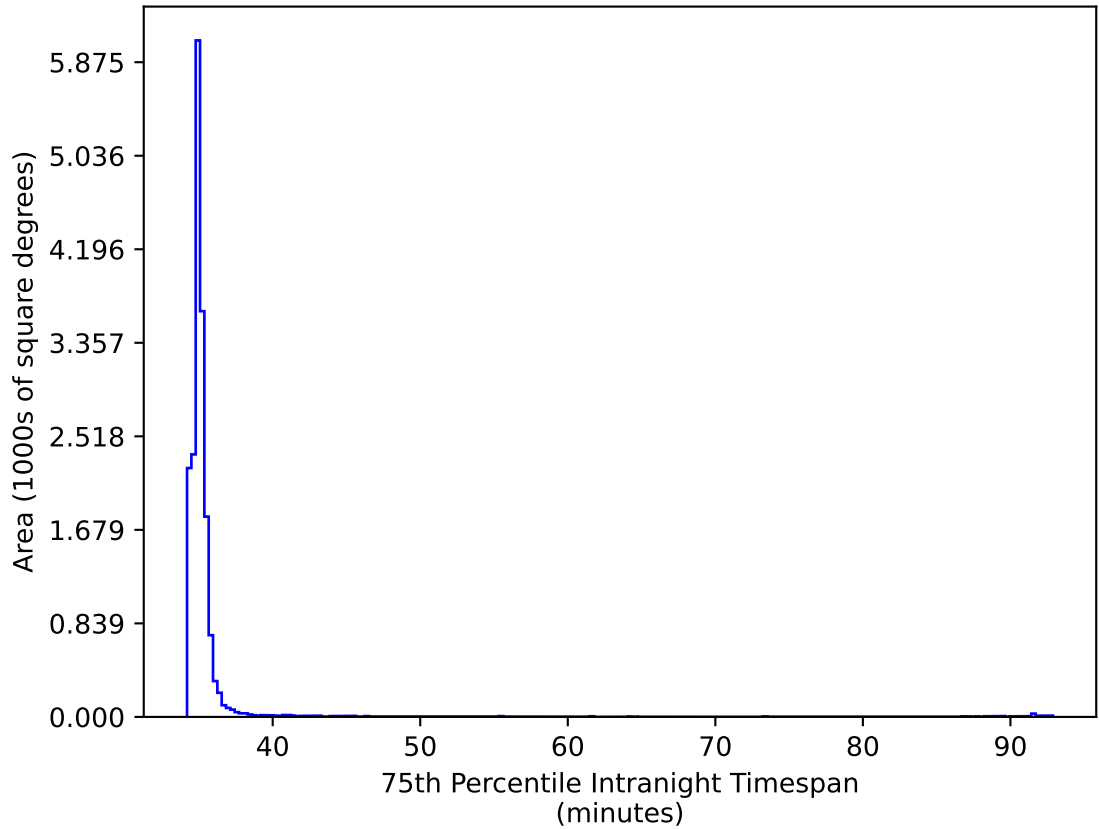
too_ignore_5_1v3.4_10yrs WFD ri bands: 75th Percentile Intranight Timespan
