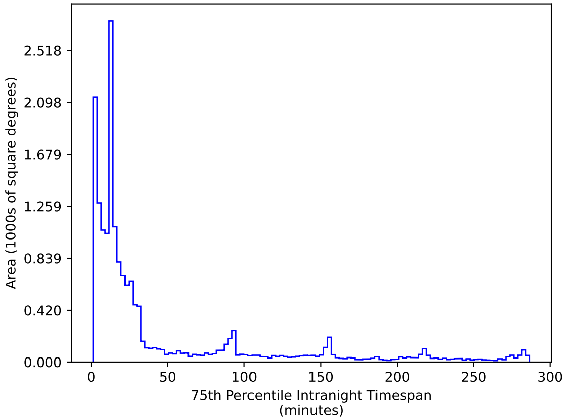
too_ignore_5_1v3.4_10yrs WFD r band: 75th Percentile Intranight Timespan
