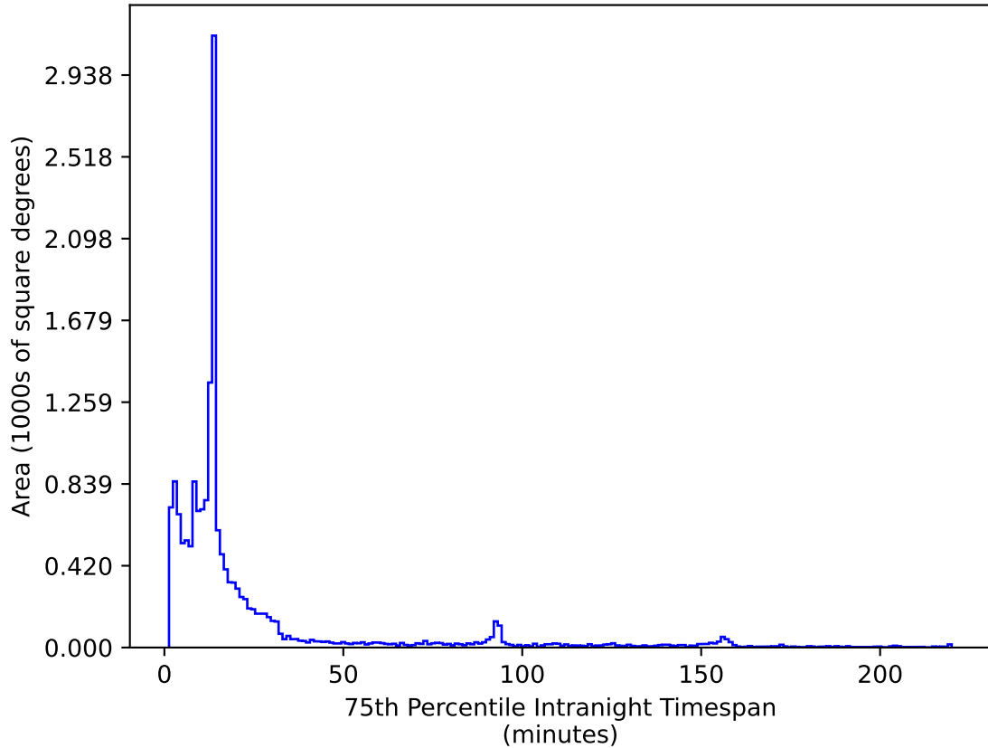
too_ignore_5_1v3.4_10yrs WFD i band: 75th Percentile Intranight Timespan
