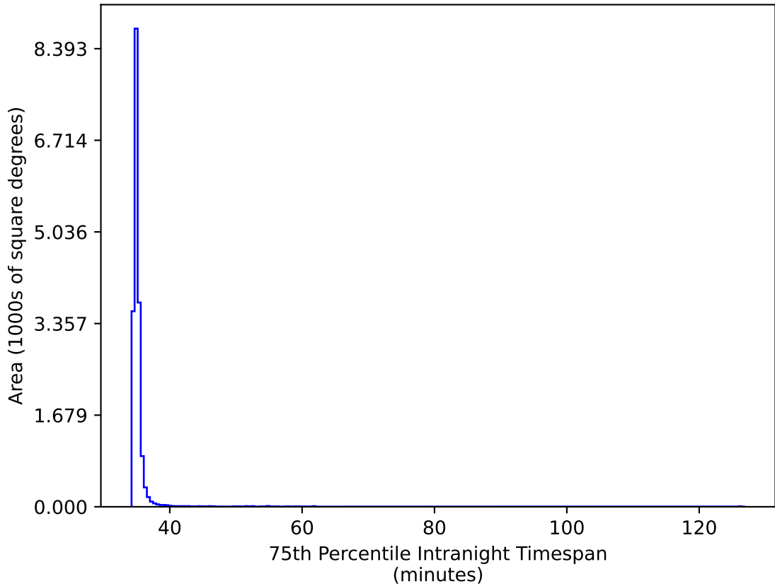
too_ignore_5_1v3.4_10yrs WFD gr bands: 75th Percentile Intranight Timespan
