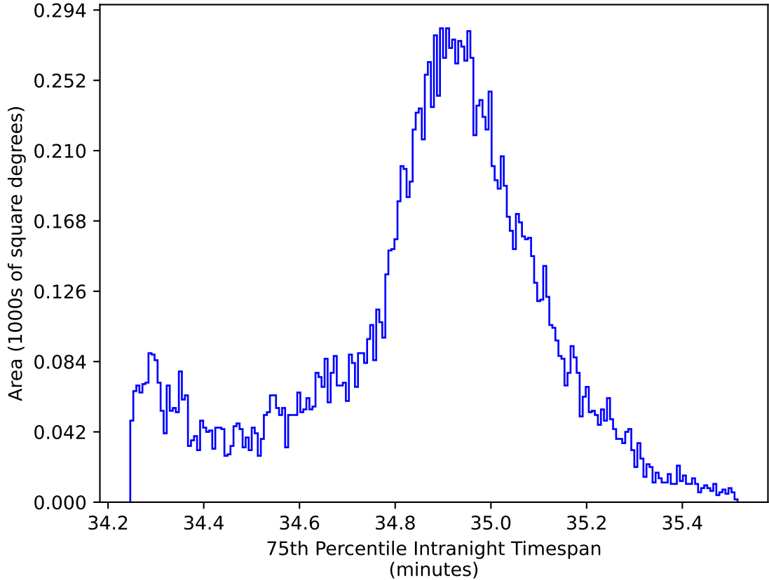
too_ignore_5_1v3.4_10yrs WFD all bands: 75th Percentile Intranight Timespan
