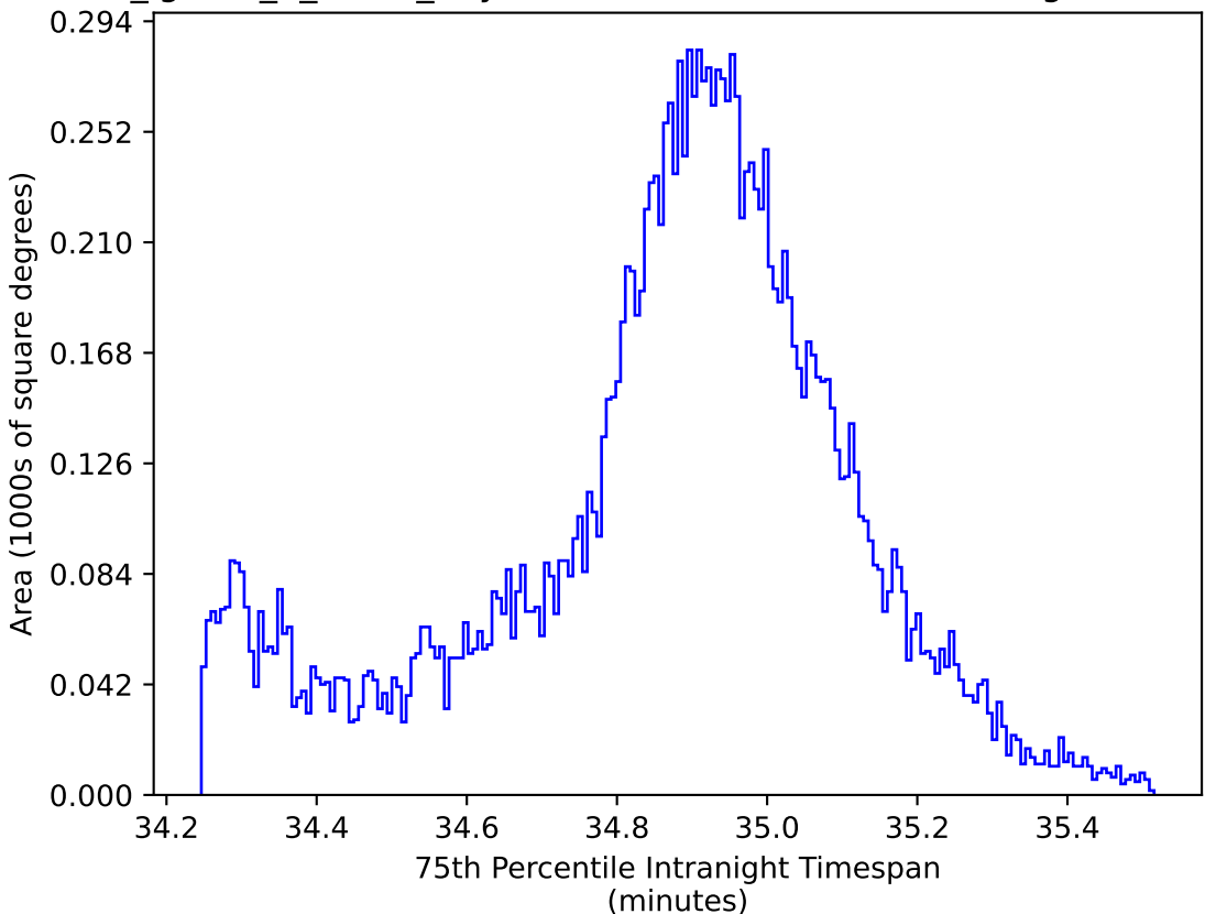
too_ignore_5_1v3.4_10yrs WFD: 75th Percentile Intranight Timespan
