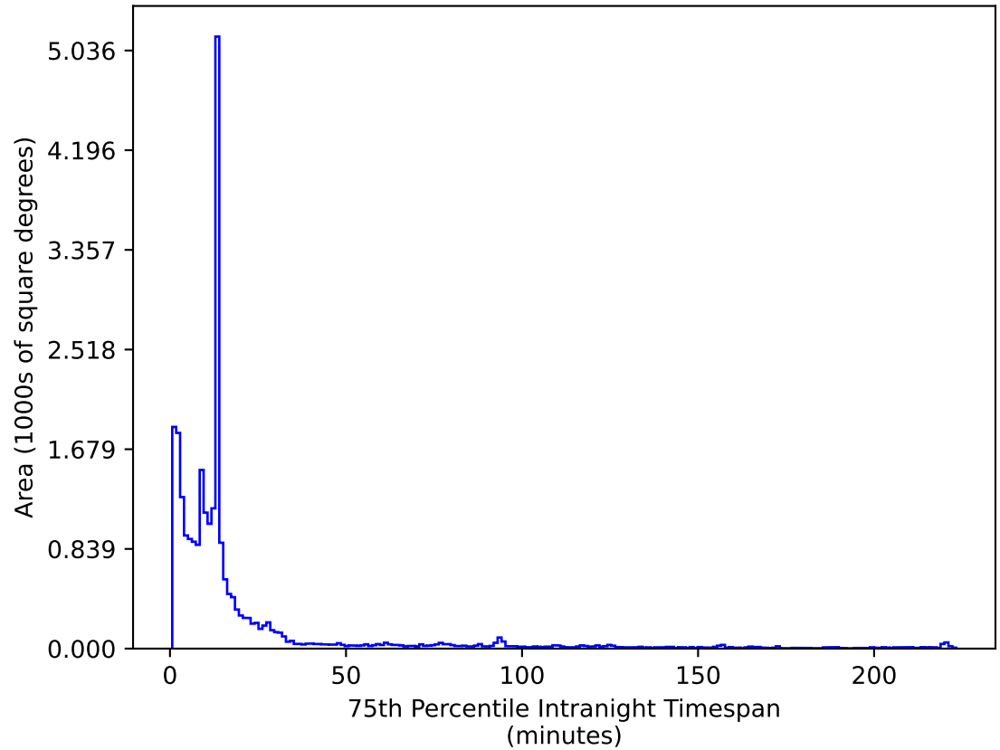
too_ignore_5_1v3.4_10yrs All sky z band: 75th Percentile Intranight Timespan
