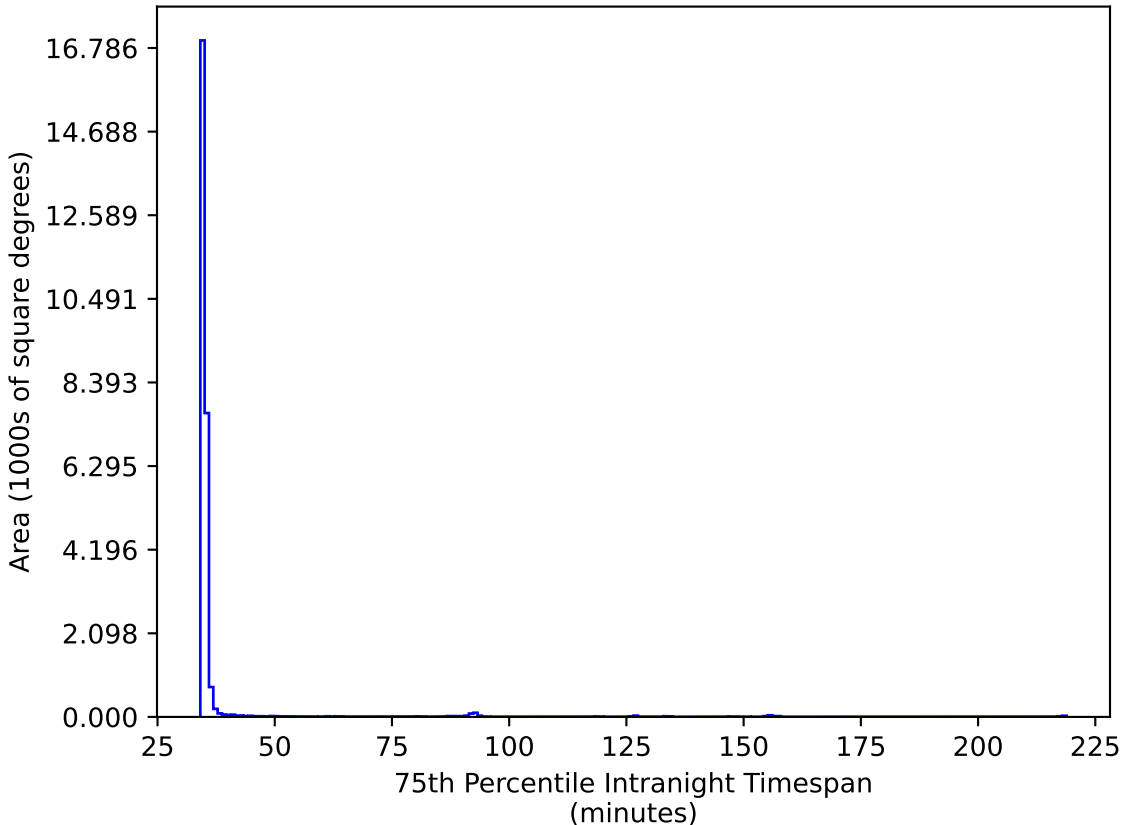
too_ignore_5_1v3.4_10yrs All sky ri bands: 75th Percentile Intranight Timespan
