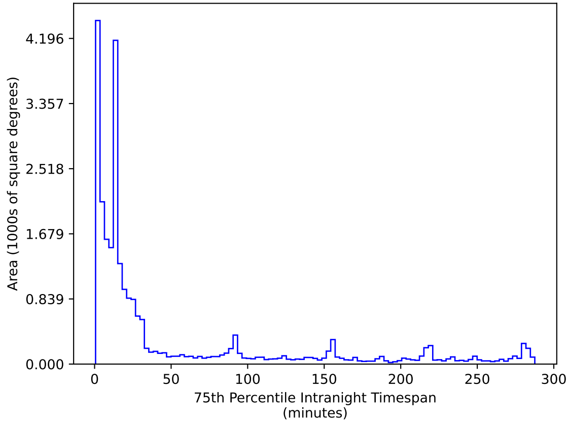
too_ignore_5_1v3.4_10yrs All sky r band: 75th Percentile Intranight Timespan
