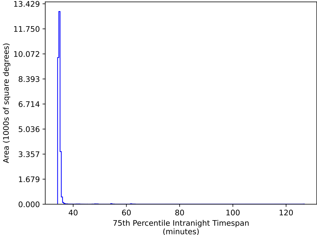
too_ignore_5_1v3.4_10yrs All sky iz bands: 75th Percentile Intranight Timespan
