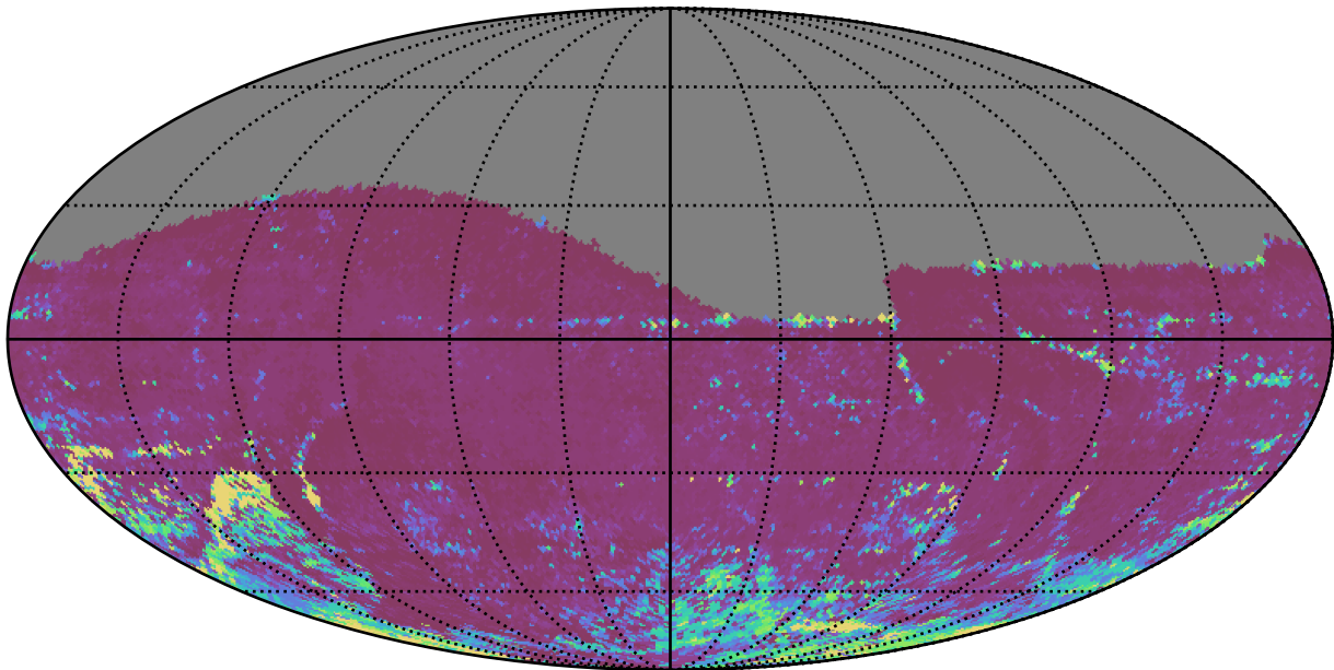
too_ignore_5_1v3.4_10yrs All sky i band: 75th Percentile Intranight Timespan
