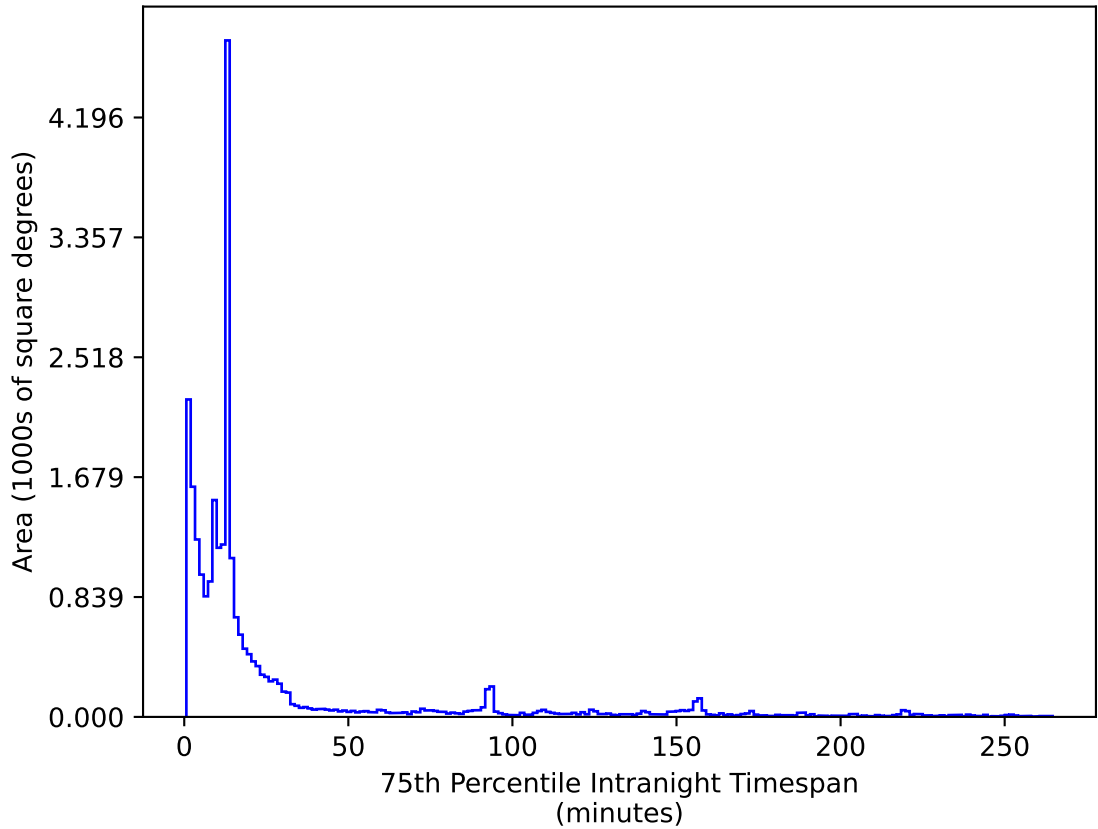
too_ignore_5_1v3.4_10yrs All sky i band: 75th Percentile Intranight Timespan
