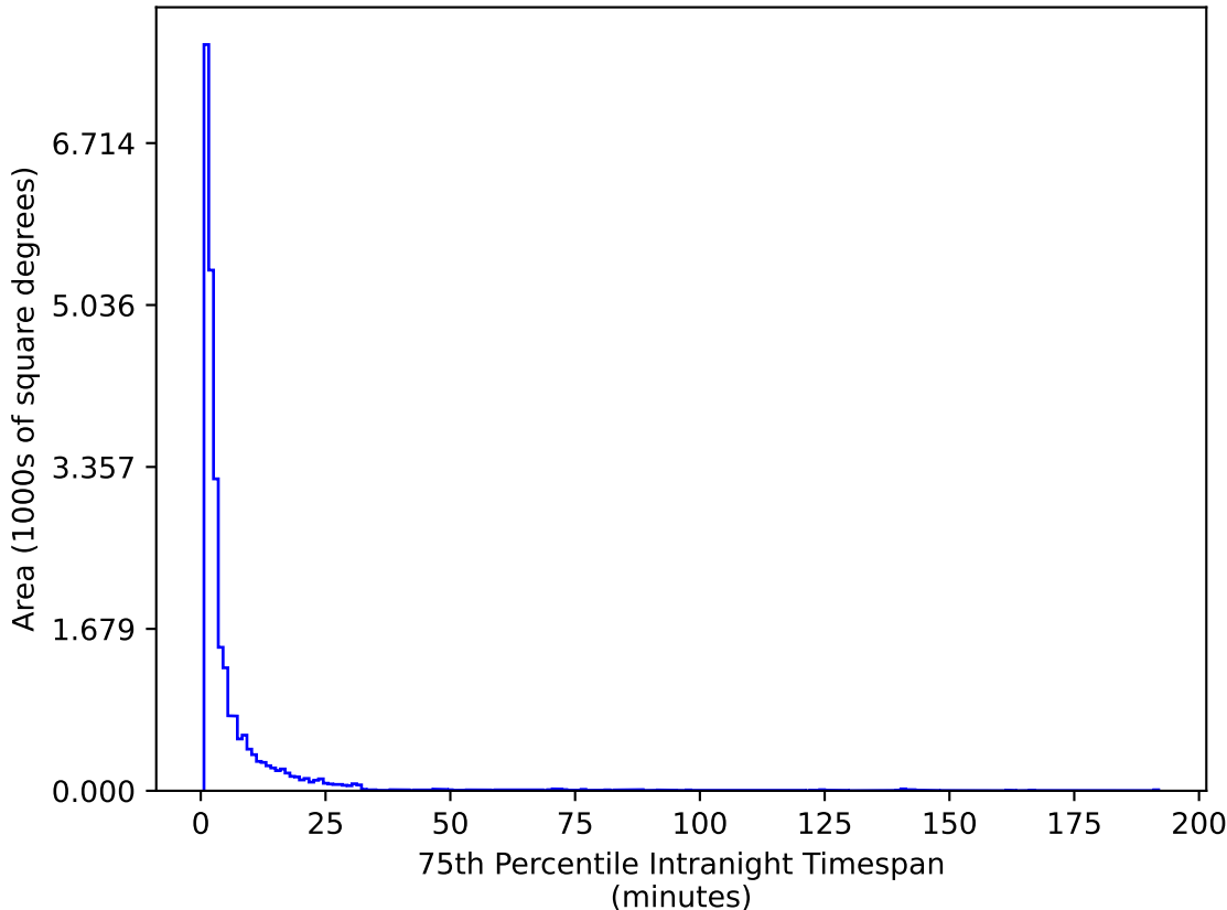
too_ignore_5_1v3.4_10yrs All sky g band: 75th Percentile Intranight Timespan
