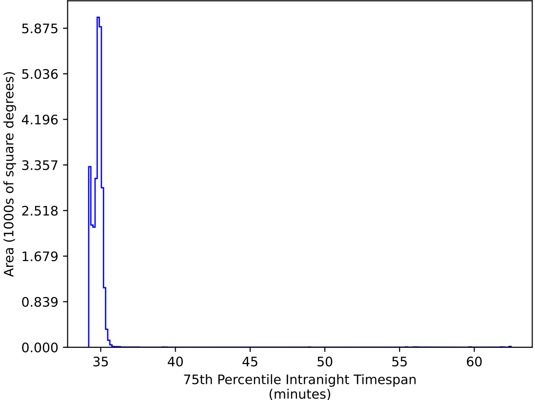
too_ignore_5_1v3.4_10yrs All sky all bands: 75th Percentile Intranight Timespan
