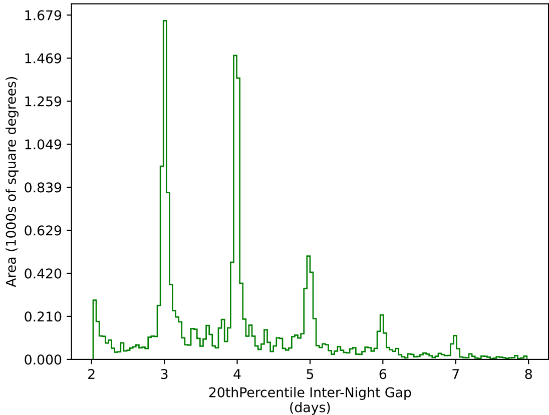
too_ignore_5_1v3.4_10yrs WFD g band: 20thPercentile Inter-Night Gap
