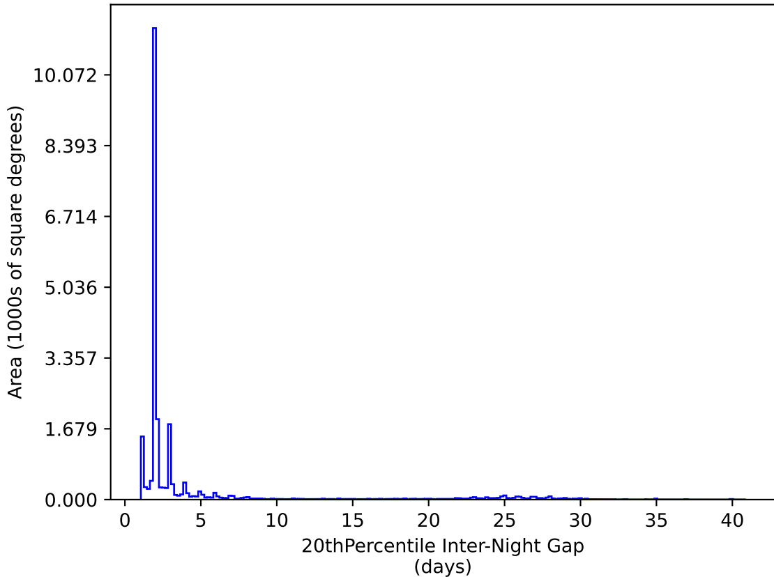
too_ignore_5_1v3.4_10yrs All sky y band: 20thPercentile Inter-Night Gap
