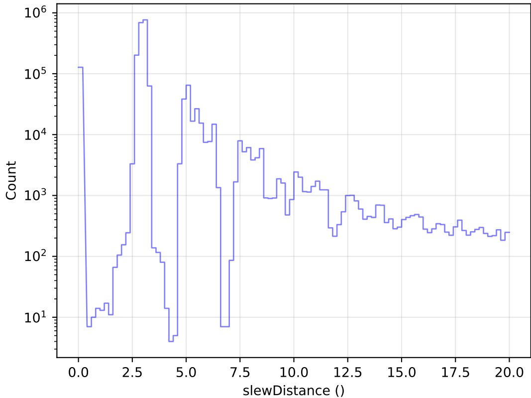
too_ignore_5_1v3.4_10yrs All visits: Zoom Slew Distance Histogram
