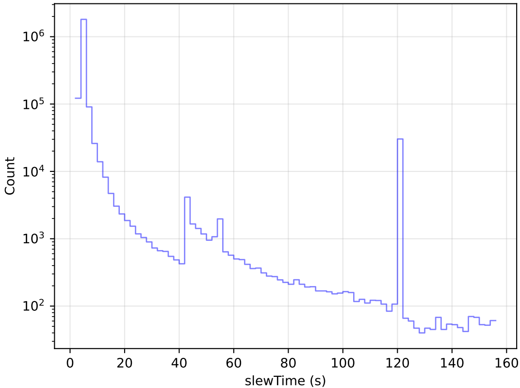
too_ignore_5_1v3.4_10yrs All visits: Slew Time Histogram
