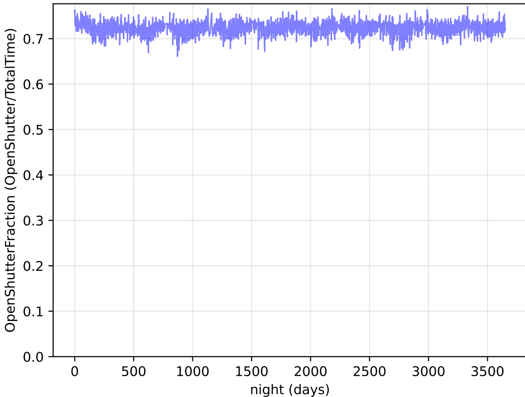
too_ignore_5_1v3.4_10yrs : OpenShutterFraction
