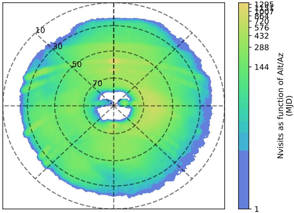
too_ignore_5_1v3.4_10yrs g: Nvisits as function of Alt/Az
