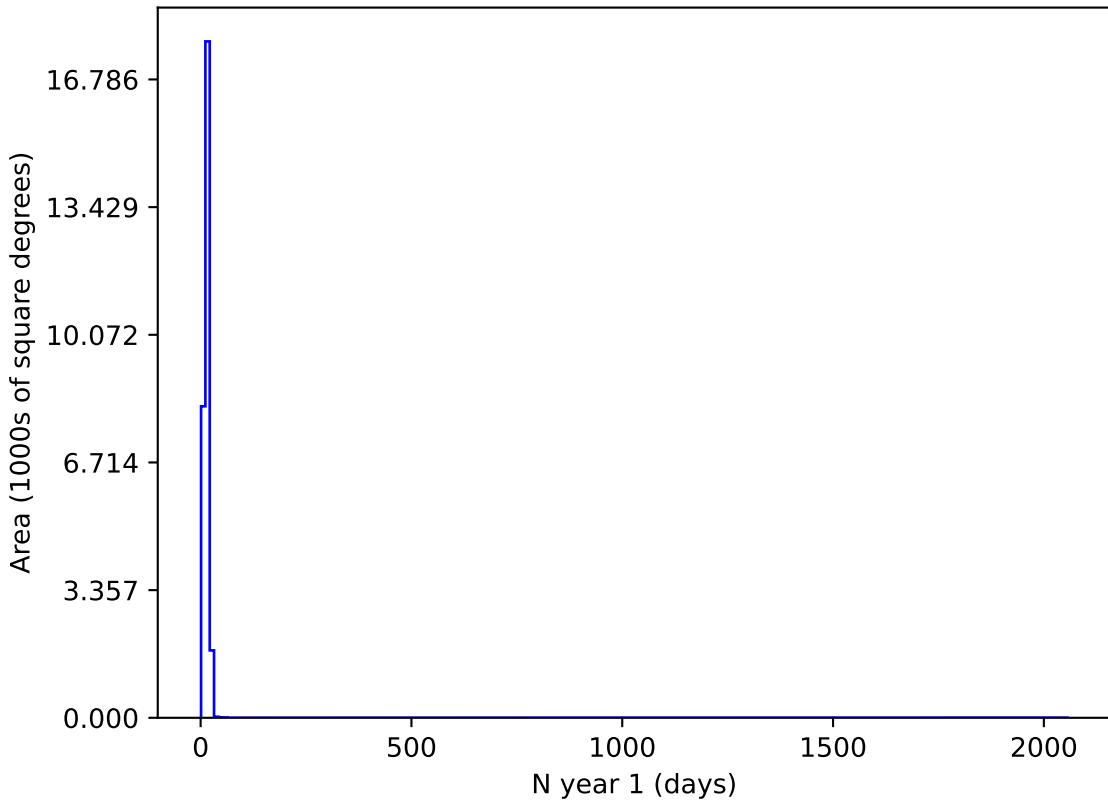
too_ignore_5_1v3.4_10yrs z and night < 365: N year 1
