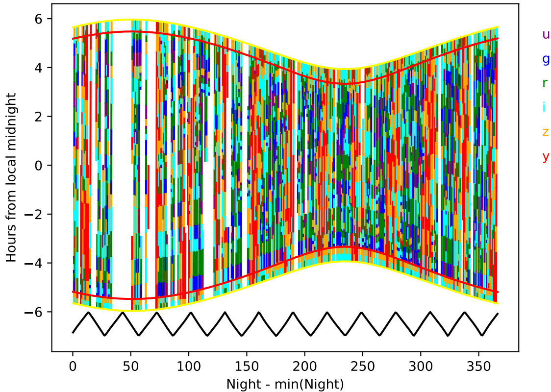
too_ignore_5_1v3.4_10yrs year 8-9: Hourglass
