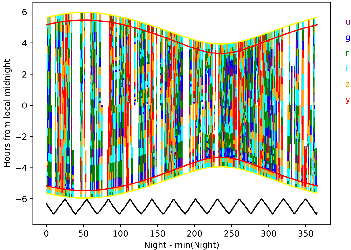
too_ignore_5_1v3.4_10yrs year 7-8: Hourglass
