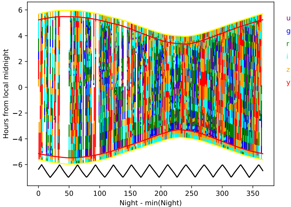
too_ignore_5_1v3.4_10yrs year 6-7: Hourglass
