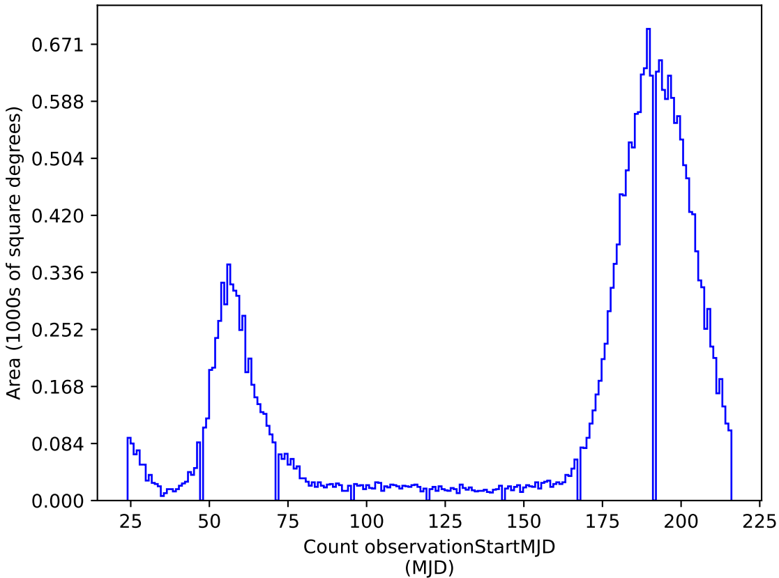
too_ignore_5_1v3.4_10yrs i: Count observationStartMJD
