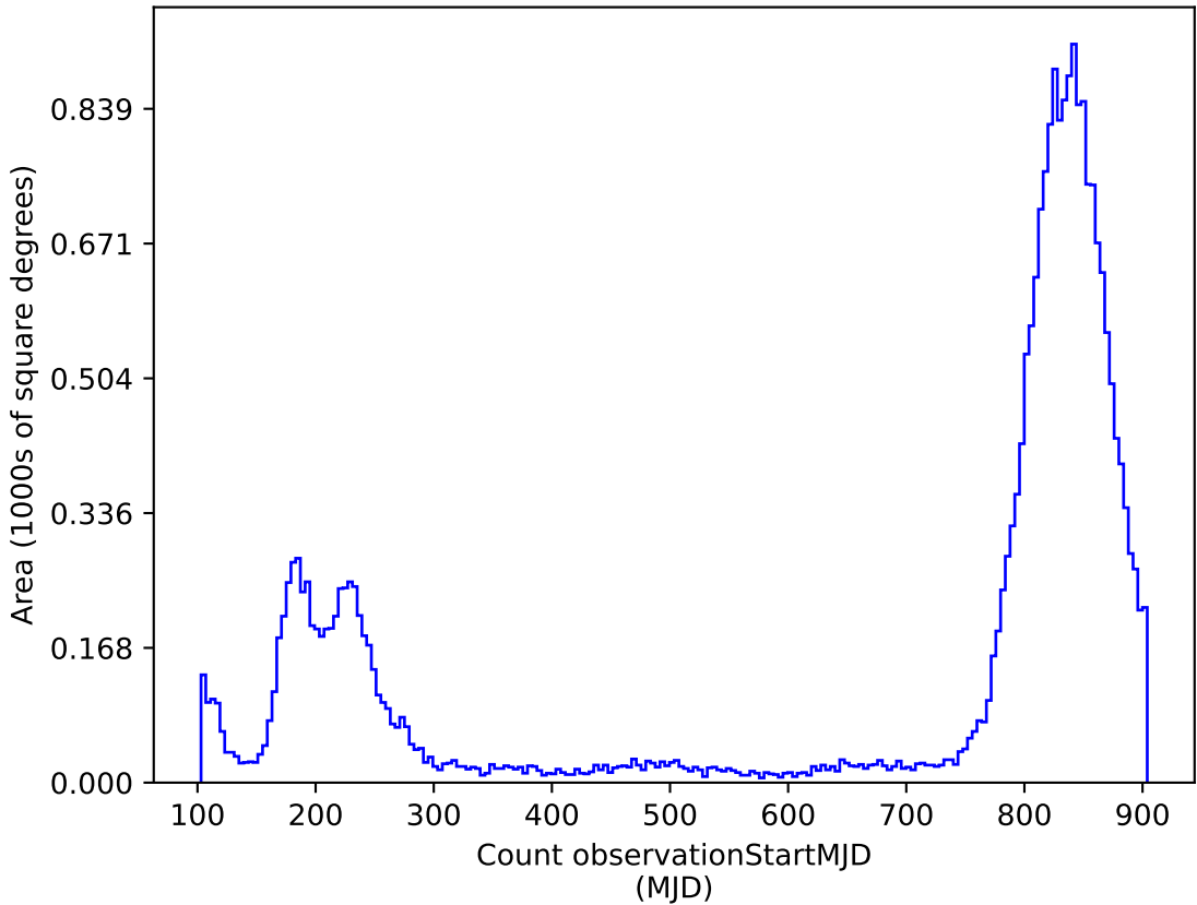
too_ignore_5_1v3.4_10yrs : Count observationStartMJD
