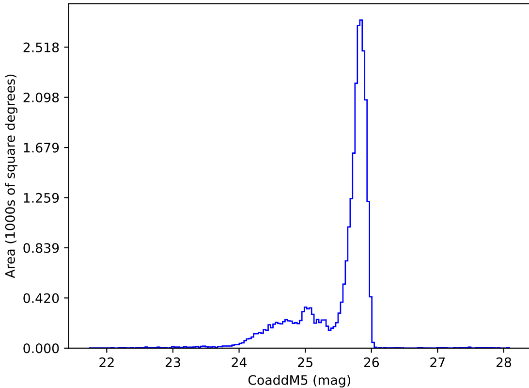
too_ignore_5_1v3.4_10yrs z: CoaddM5
