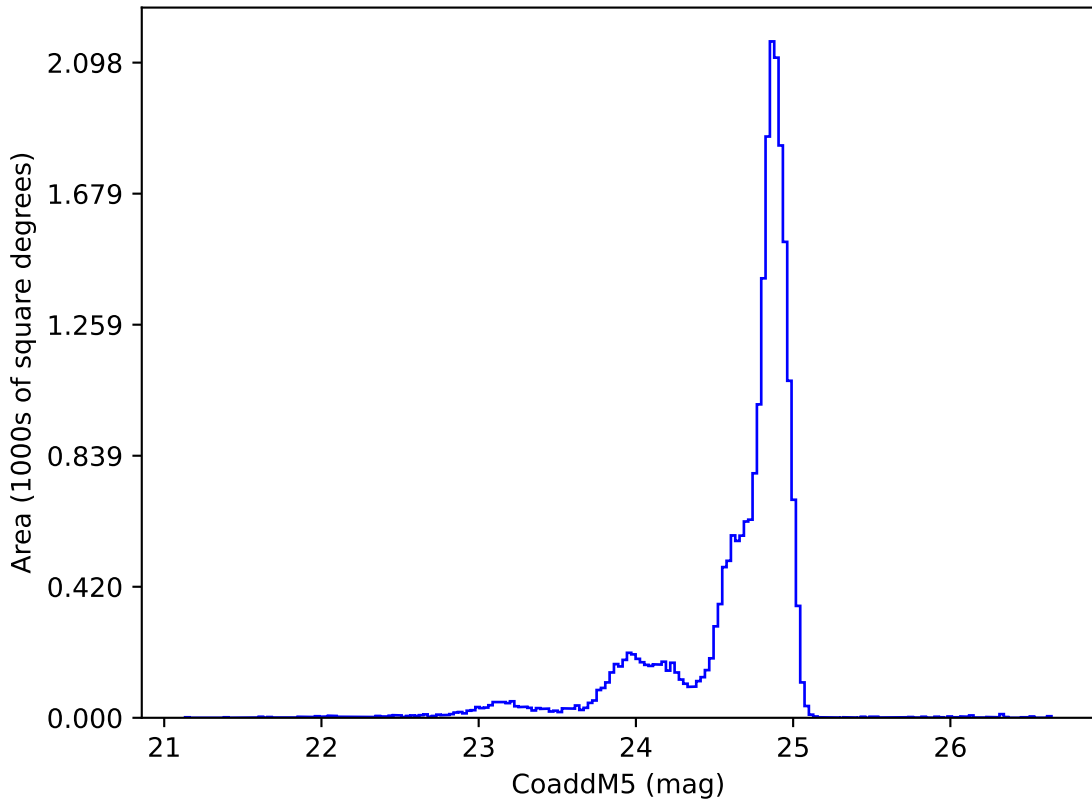
too_ignore_5_1v3.4_10yrs y: CoaddM5
