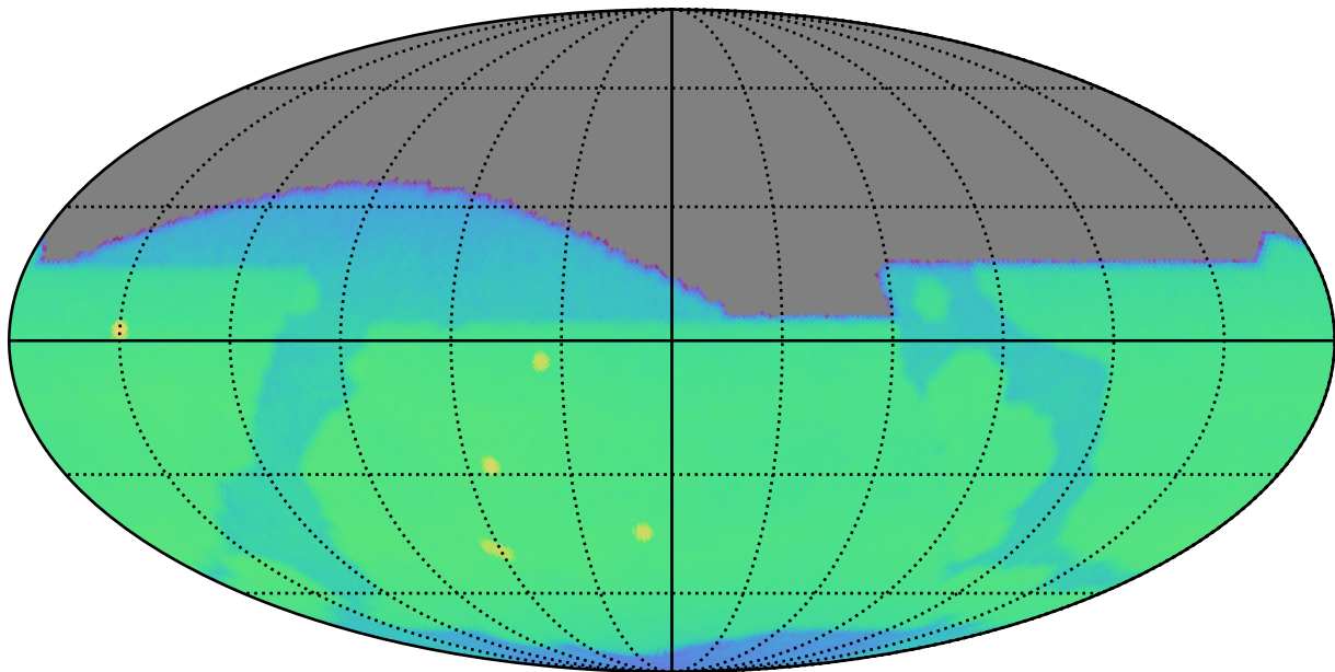
too_ignore_5_1v3.4_10yrs r: CoaddM5
