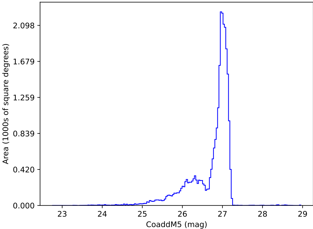
too_ignore_5_1v3.4_10yrs r: CoaddM5
