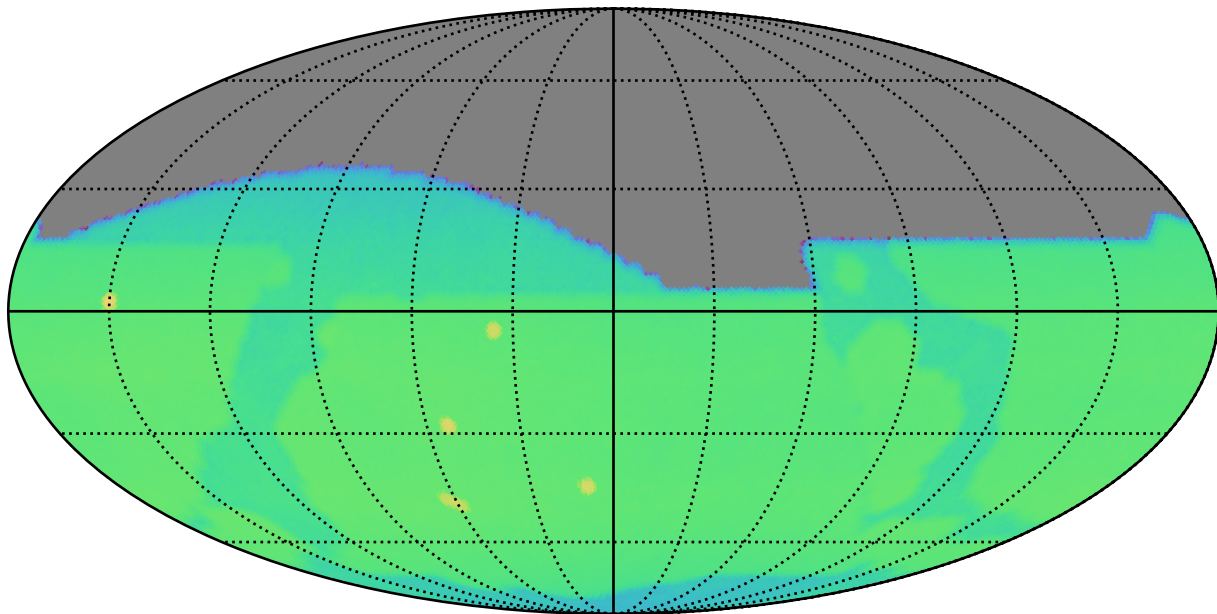
too_ignore_5_1v3.4_10yrs : CoaddM5
