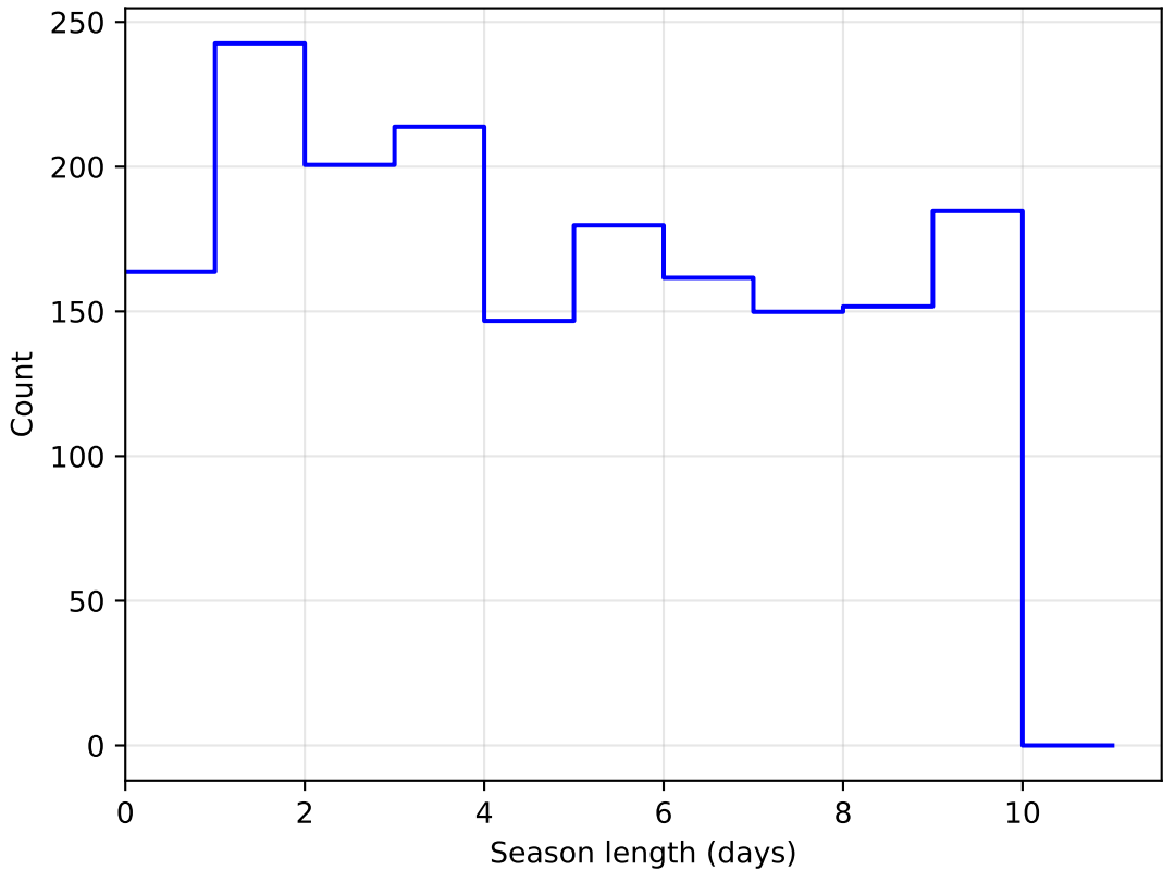
too_ignore_5_1v3.4_10yrs DD:WFD all bands: SeasonLength
