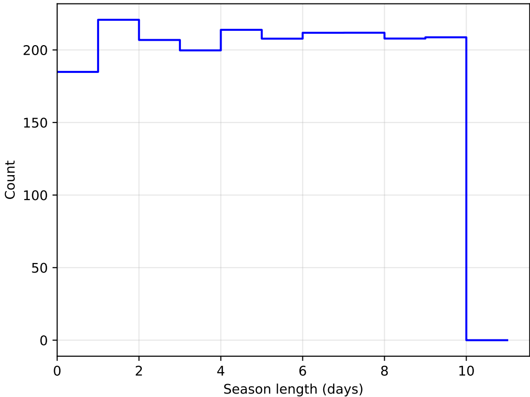
too_ignore_5_1v3.4_10yrs DD:ELAISS1 all bands: SeasonLength
