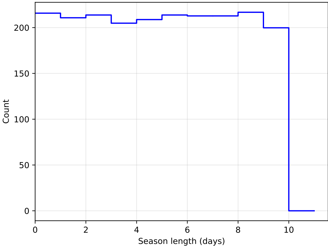
too_ignore_5_1v3.4_10yrs DD:ECDFS all bands: SeasonLength
