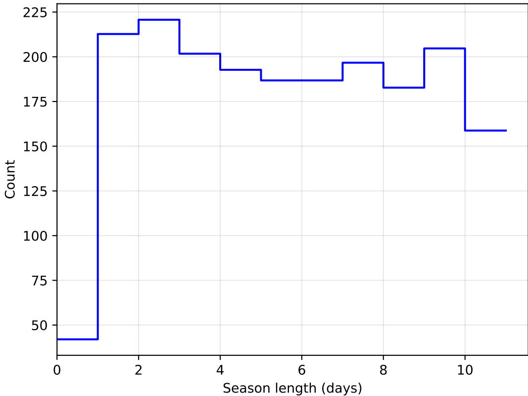
too_ignore_5_1v3.4_10yrs DD: COSMOS all bands: SeasonLength
