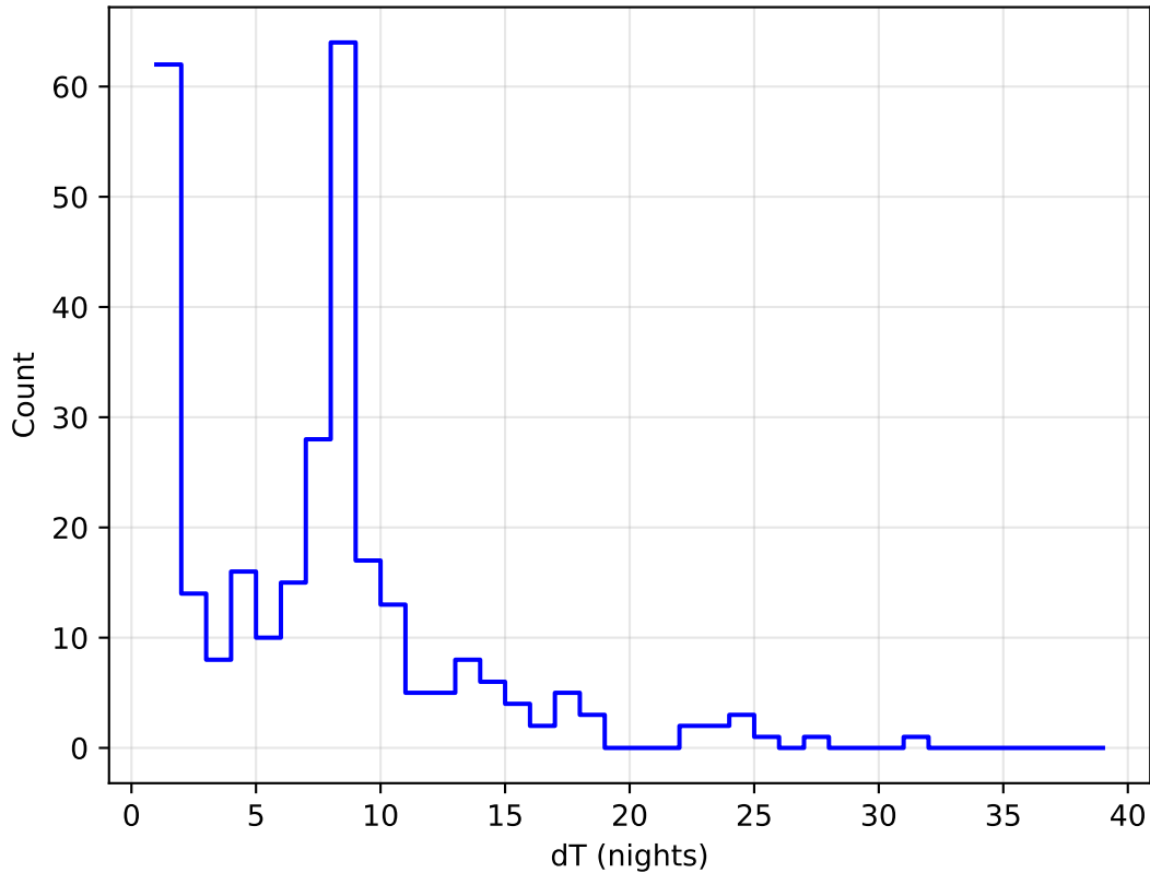
too_ignore_5_1v3.4_10yrs all bands: DD:XMM_LSS Delta Nights Histogram
