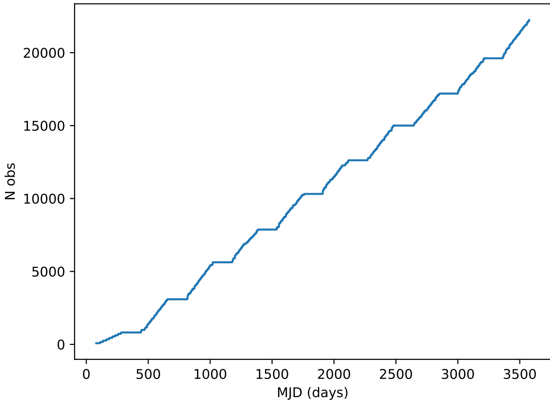
too_ignore_5_1v3.4_10yrs all bands: DD:XMM_LSS Cumulative NVisits
